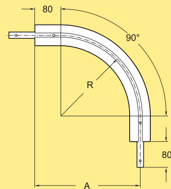
Vertical bend, 90° R= 400, A= 480 XHBV 90R400 R=1000, A=1080 XHBV 90R1000 Effective track length: R400: 0,85 m 1-way (1,60 m 2-way) R1000: 1,75 m 1-way (3,50 m 2-way)
