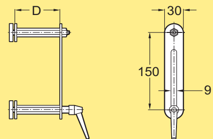
Bend support D=43 mm D=93 mm
