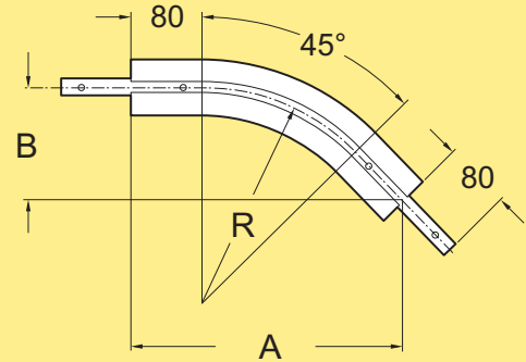
Vertical bend, 45° R= 400, A=419, B=174 XHBV 45R400 R=1000, A=844, B=349 XHBV 45R1000 Effective track length: R400: 0,50 m 1-way (0,95 m 2-way) R1000: 0,95 m 1-way (1,90 m 2-way)
